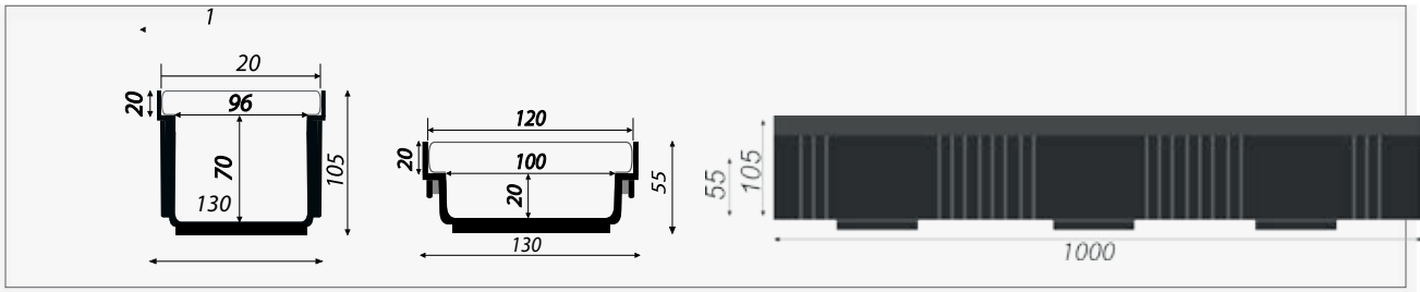
Technical sections of linear drain
